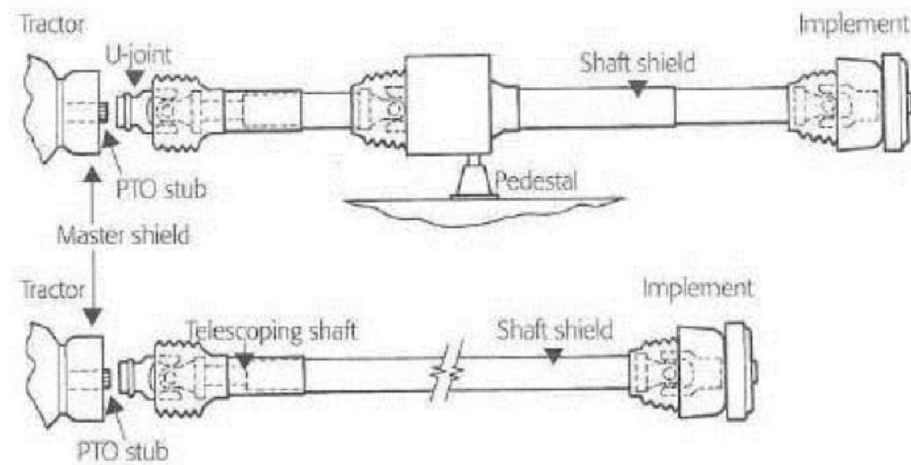
Fig. 1. PTO components
